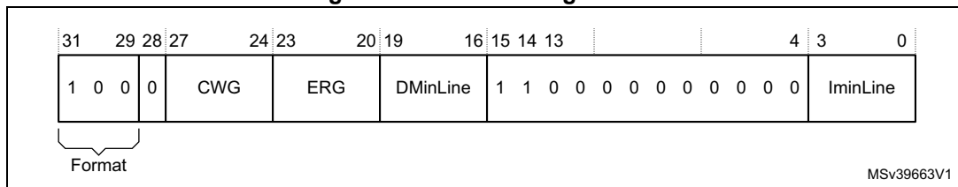
Figure 45. CTR bit assignments
