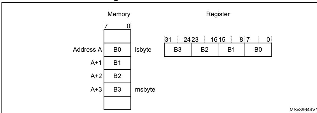
Figure 9. Little-endian format
