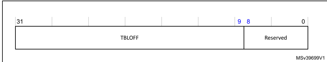
Figure 27. VTOR bit assignments
