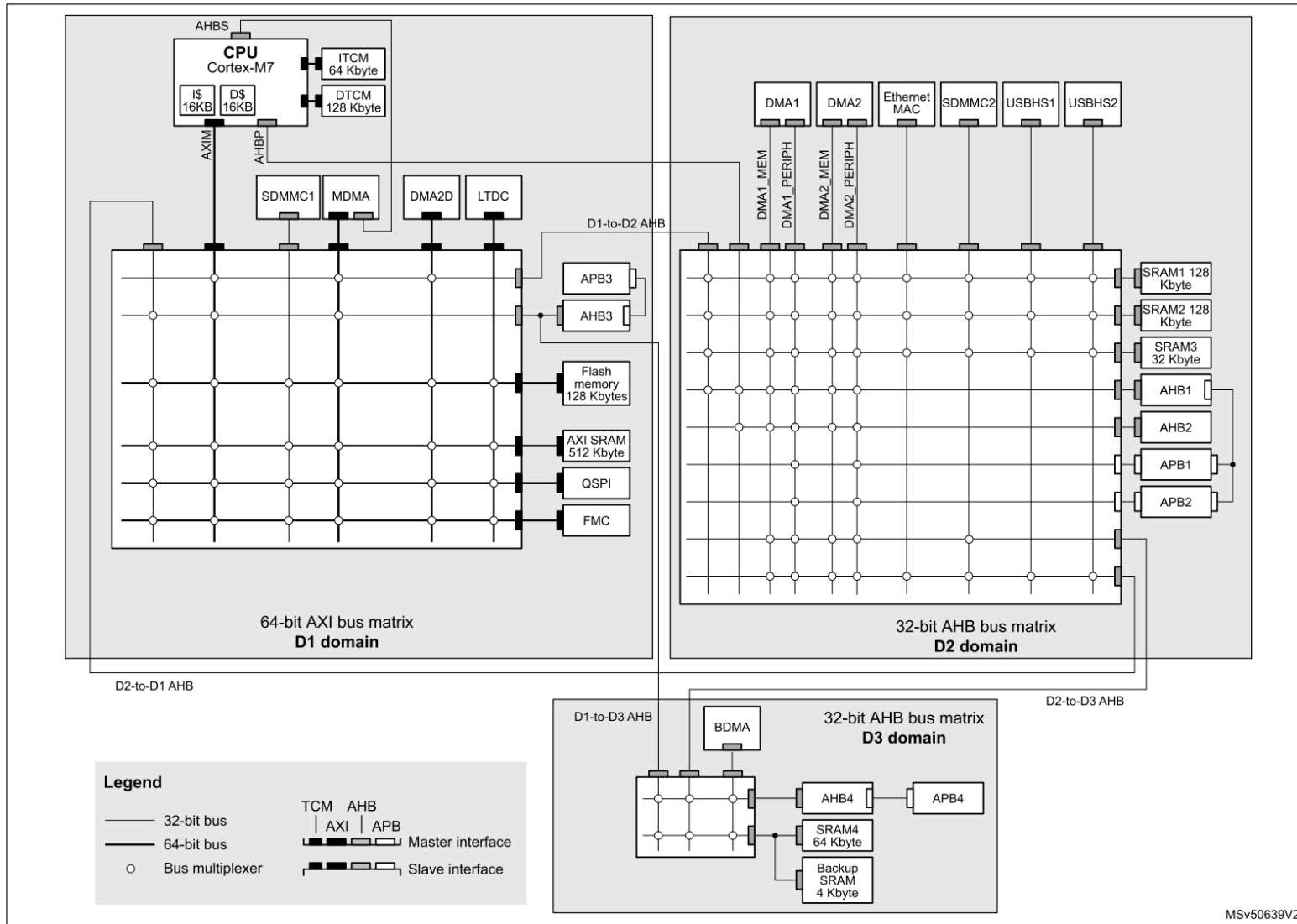
Figure 3. STM32H750xB bus matrix
