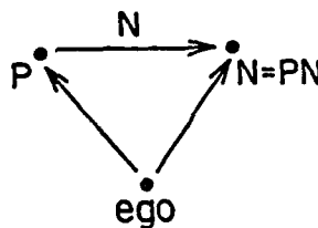
FIGURE 10 Roles related by a role relation.
