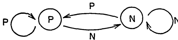
FIGURE 9 Graphic representation of the composition operation in Figure 8.
