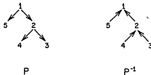
FIGURE 1 A hierarchical tree.
