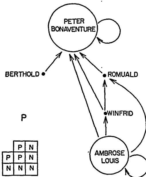
FIGURE 7 A first example of reduction of the network of Figure 6. Only the graph of P is shown; the graph of N is a trivial one linking every node to every other node.
