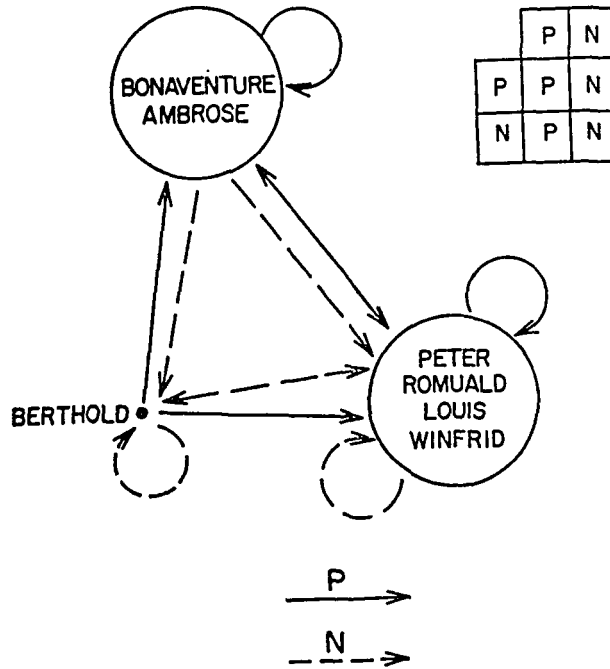
FIGURE 8. A second example of reduction of the network of Figure 6.
