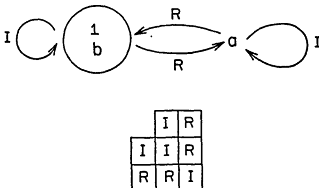
FIGURE 11 A reduction of the category of Figure 5 and Table 5.
