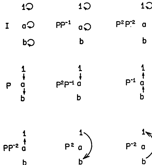
FIGURE 4 Graphs of morphisms in the reduction of the network of Figure 1, implied by the identification P^{-1}P \equiv I . a represents the set of nodes 2 and 5, b the set of nodes 3 and 4.
