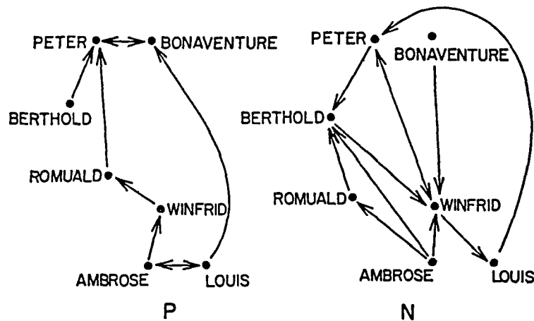
FIGURE 6 Positive and negative relations in a monastery.
