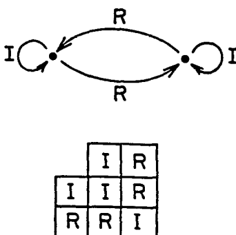
FIGURE 12 The two-category: the graph of the cyclic group of order two. This category is isomorphic to the one in Figure 11.
