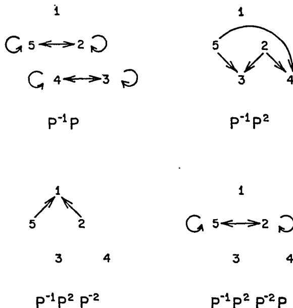
FIGURE 2 Graphs of four of the types of relation in Table 1
