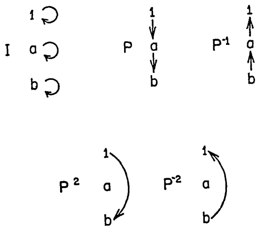
FIGURE 5 Graphs of morphisms in the reduction of the network of Figure 1, implied by the identifications PP^{-1} \equiv P^{-1}P \equiv I . a and b as in Figure 4.
