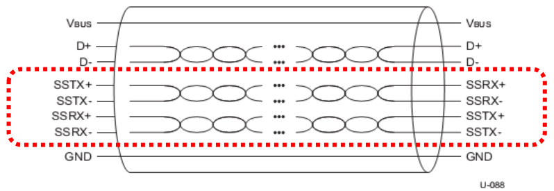
Figure 3-2. USB 3.0 Cable
