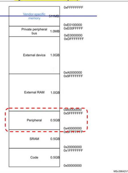
Figure 8. Processor memory map
